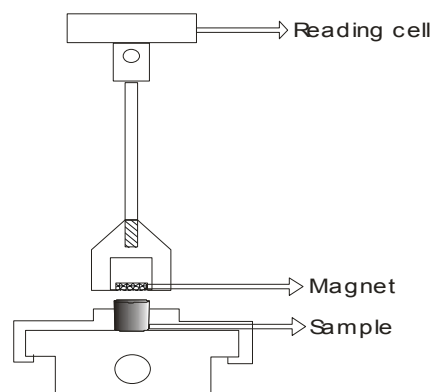
Figure 1 - Magnetic traction apparatus
